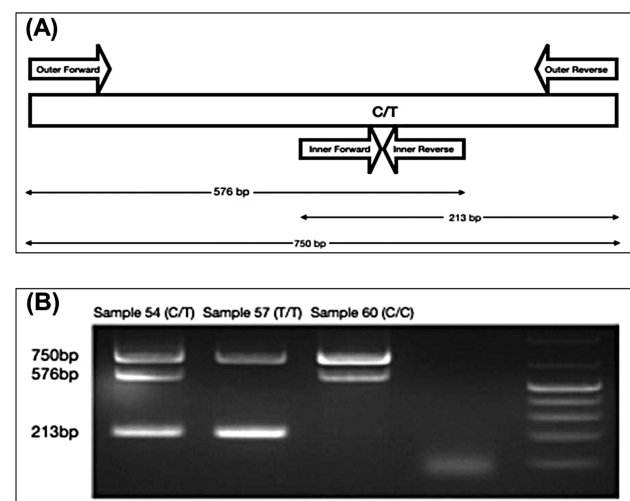
Fig. 1 Schematic illustration of tetra-ARMS PCR assay for SNP rs13041247 genotyping. (A) Location of primers and SNP rs13041247. (B) Agarose gel electrophoresis image of PCR products. T/T, homozygote for the allele T; C/C, homozygote for the allele C; C/T, heterozygote for the alleles C and T; SNP, single-nucleotide polymorphism; tetra-ARMS PCR, tetra-amplification refractory mutation system polymerase chain reaction.
